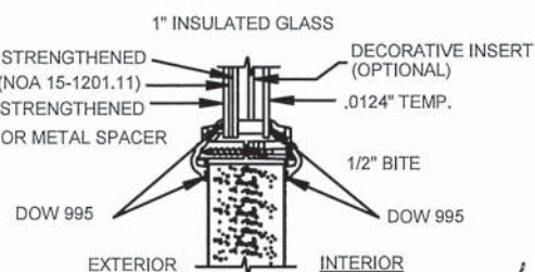
TYPICAL GLAZING DETAIL IMPACT RATED GLASS
