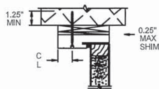
1X BUCK MASONRY ANCHOR INSTALLATION Addendum to Certification
