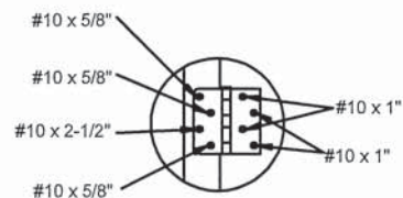
DETAIL "C"
